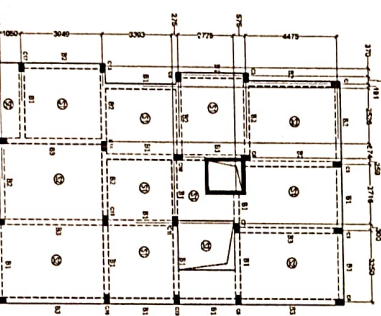
TYPICAL BEAM ARRANGEMENT PLAN Designed by ZWCAD Academic Version
